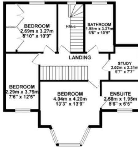
1ST FLOOR 64.89 sq. m. ( 698.45 sq. ft. )
