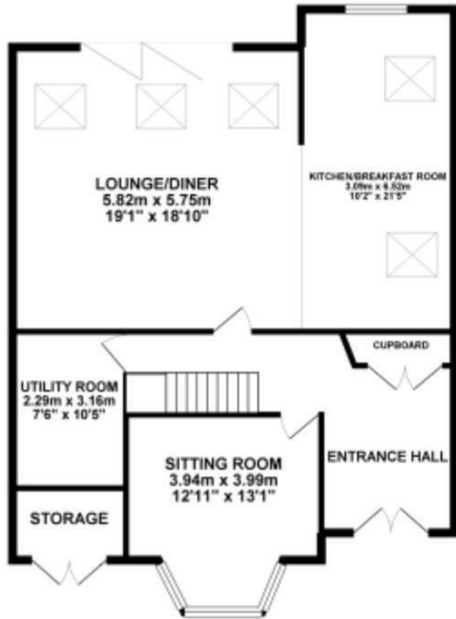
GROUND FLOOR 95.45 sq. m. ( 1027.44 sq. ft. )
